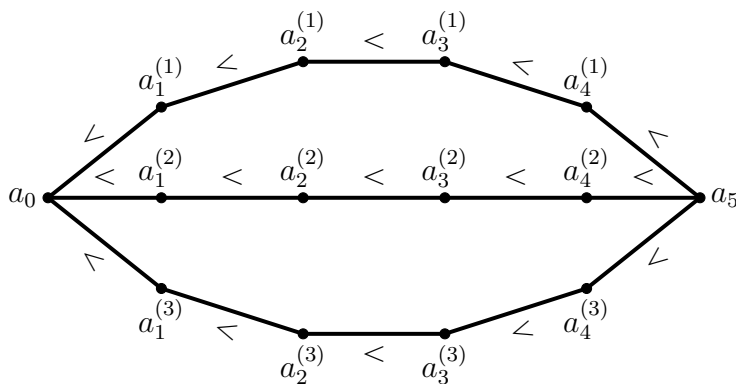
FIGURE 2.1. Ordered theta graph \Theta_{5,3} .
