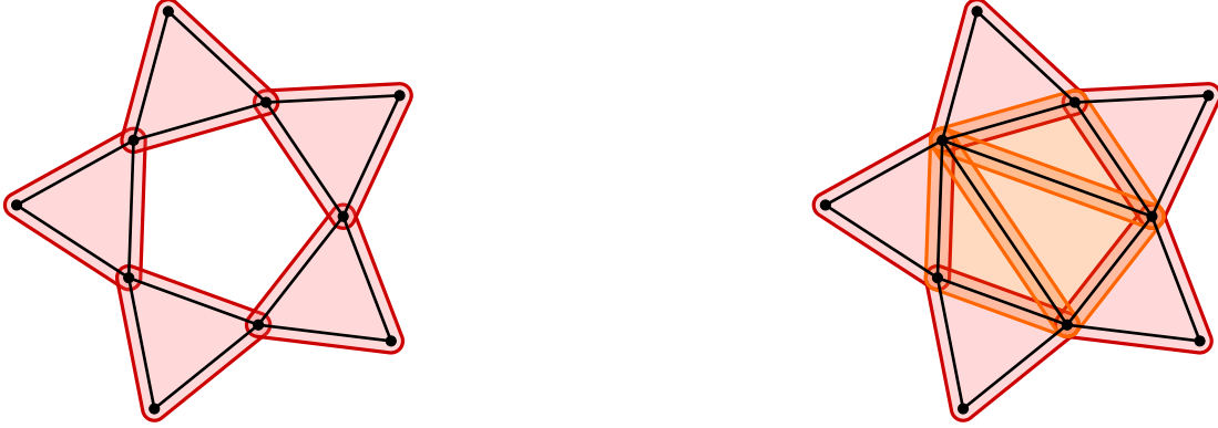
(a) A ‘cycle’ of triangles ...
