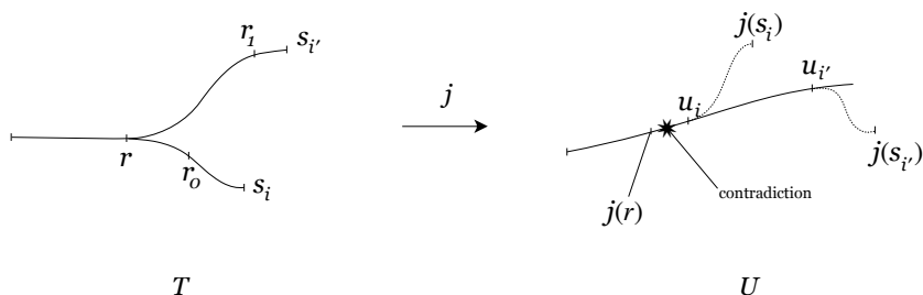
Figure 1. Contradiction assuming s_i \perp s_{i'} .
